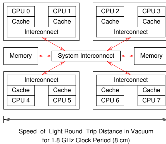
Figure 7.7: System Architecture and Lock Unfairness
