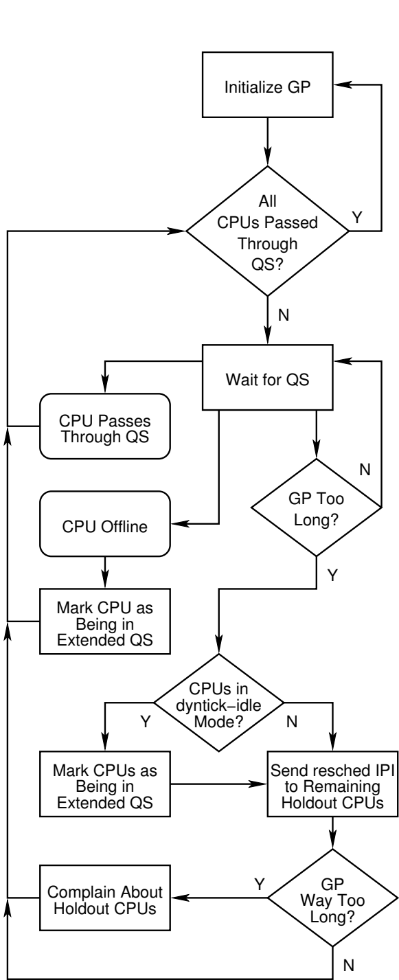
Figure D.18: Generic RCU State Machine
