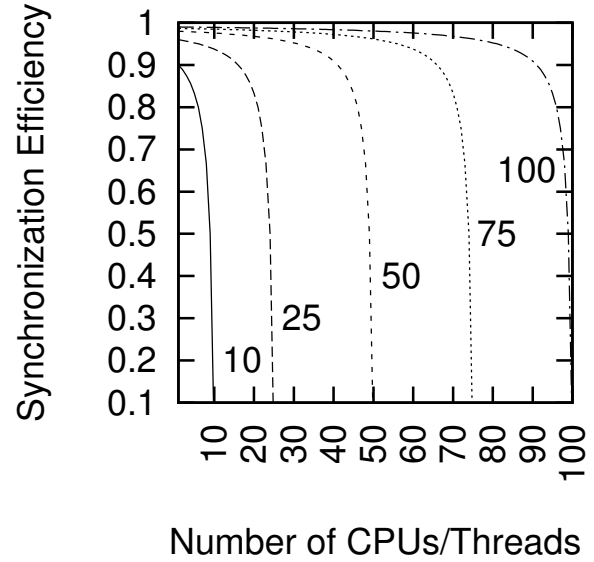
Figure 5.21: Synchronization Efficiency
