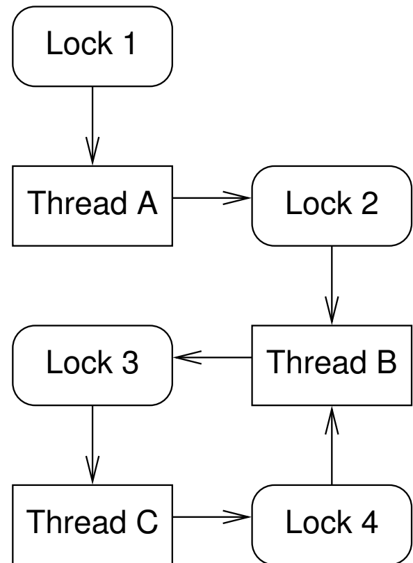
Figure 6.3: Deadlock Cycle
